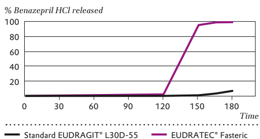
Comparative dissolution profile of Benazepril HCl pellets with Buffer of pH 5.5 commencing at 120 minutes
