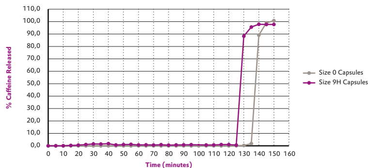
Dissolution profile of caffeine:lactose filled capsules EUDRACAP® preclinic enteric (purple) and EUDRACAP® enteric (grey).
